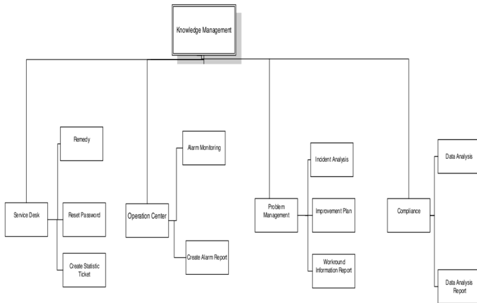
Fig. 1: Knowledge Taxonomy
