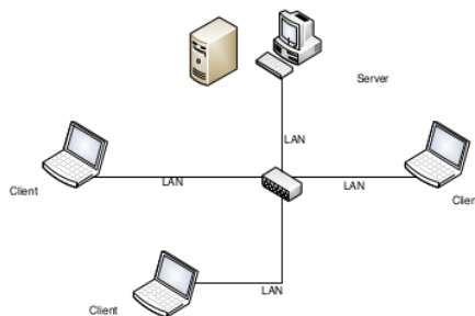
Fig. 4: Network Architecture
