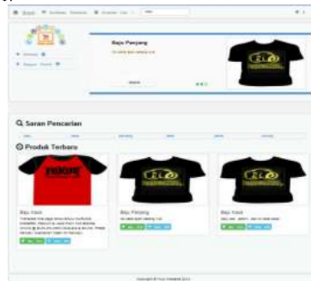
Fig. 11 Searching Page
